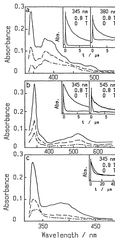
Fig. 3. Transient absorption spectra of bifunctional chain molecules. (a) AQ-12-XH in benzene. Delaytimes are 0.12 (—), 0.5 (----), and 1 \text{ }\mu\text{s} (— · —). (b) BP-12-XH in acetonitrile. Delaytimes are 0.25 (—), 1 (----), and 5 \text{ }\mu\text{s} (— · —). (c) AP-12-XH in acetonitrile. Delaytimes are 2 (—), 10 (----), and 20 \text{ }\mu\text{s} (— · —). Insets in the respective figures are the magnetic field effects on the decay curves of transients.
